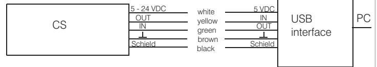
Connection diagram CS/USB programming interface
