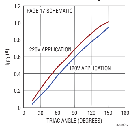
LED Current vs TRIAC Angle
